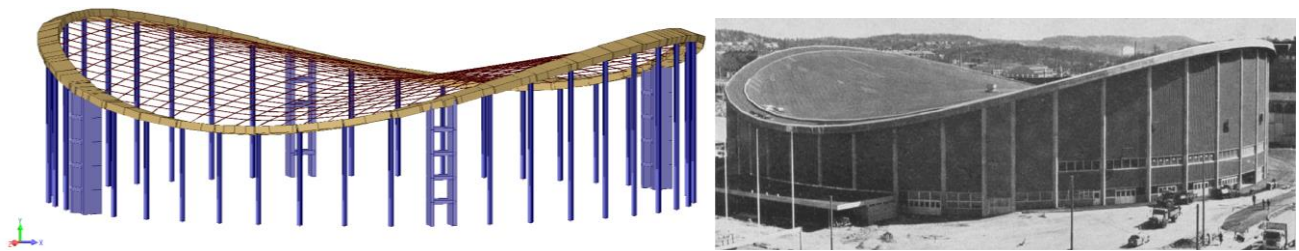
SAFI 3D Model | Scandinavium arena, Gothenburg, Sweden
