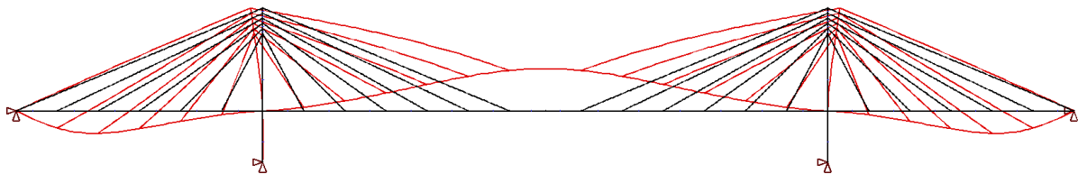
SAFI 2D Model | Meiko Nishi Bridge, Negoya, Japan (Natural frequencies Analysis)
